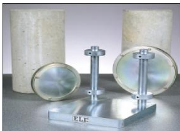
EL34-6031 Cylinder Capping Frame with Accessories
